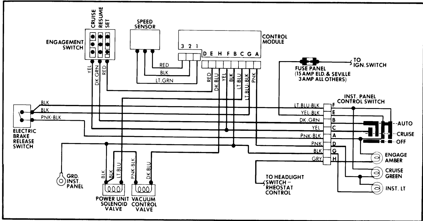
General Motors Electronic Cruise Control Automatic Speed Control System Wiring Diagram
