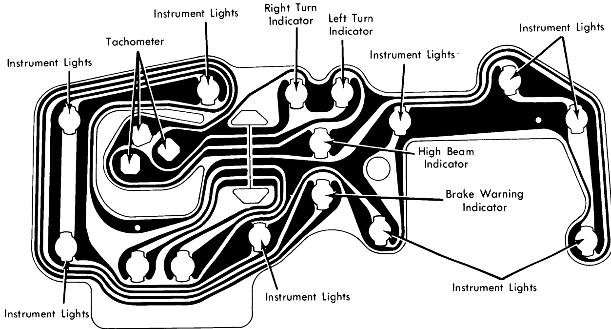
Corvette Instrument Panel Gauge Cluster
